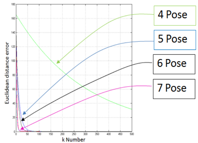
Figure 5. Convergent evolution of the algorithm.
