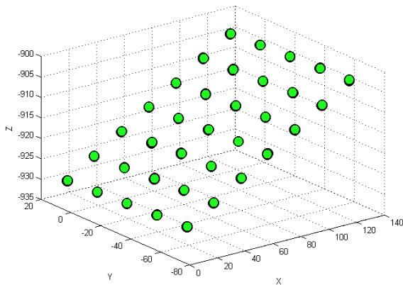
Figure 6. Position of pivot point phantom in stereo camera coordinate
